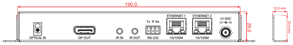
Rear View
