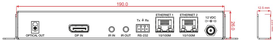
Rear View
