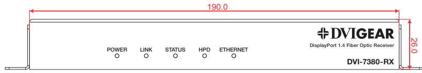
Front View
